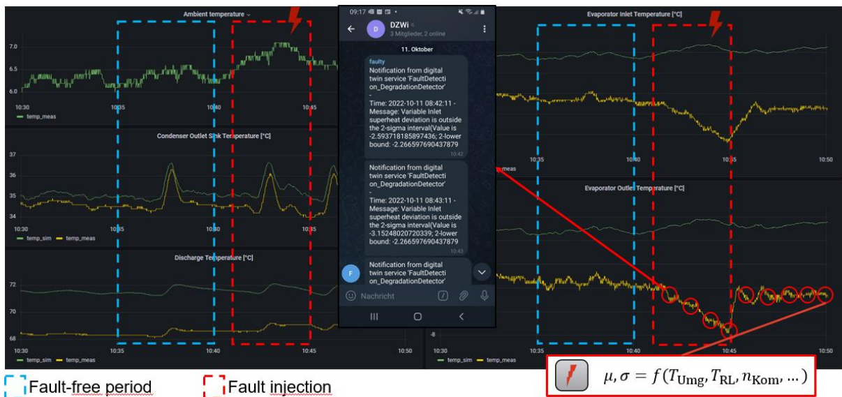
Figure 2: First results of fault detection service for evaporator fouling and resulting user notification.
