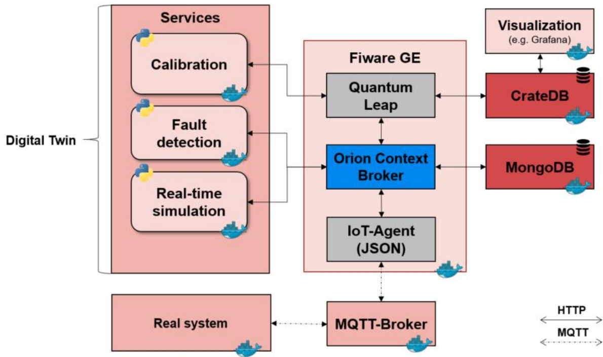
Figure 1: Fiware architecture for communication of virtual/real system and implemented services.
