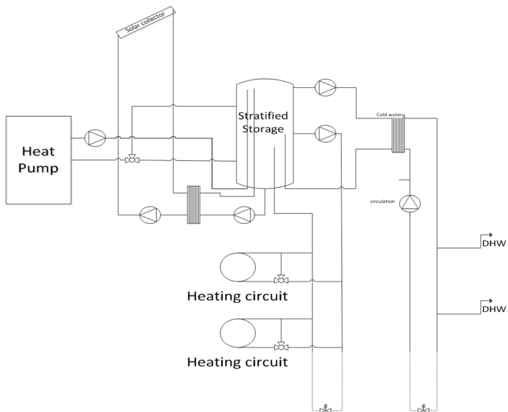
Figure 7: Simplified scheme of the hydraulic layout with centralized DHW generation (Green Heat Pump, 2014)
