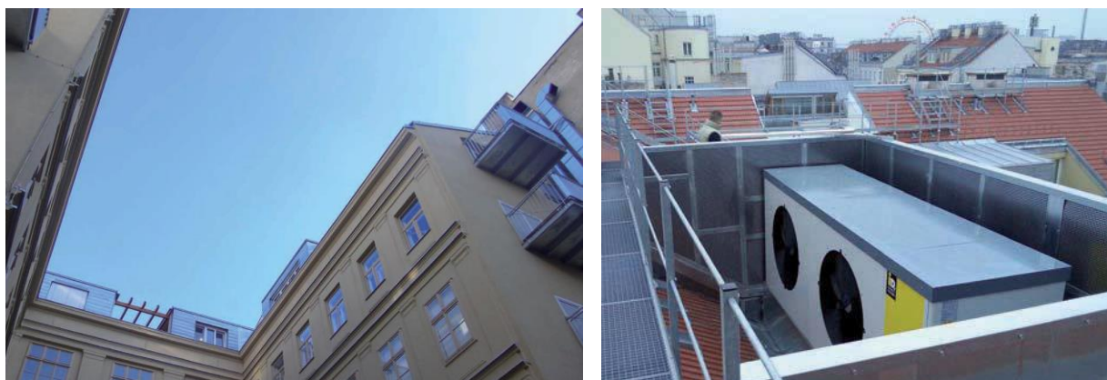
Figure 55: Pictures of the system in Wien Praterstraße (iDM Energiesysteme GmbH, 2017b)
