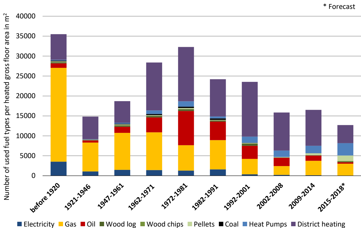
Figure 27: Number of used fuel types for heating per heated gross floor area; data according to (Invert/EE-Lab Database, 2017)
