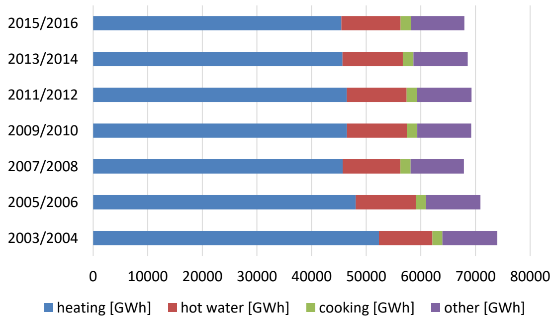
Figure 19: Final energy demand for buildings in total numbers; data according to Statistik Austria (2017)
