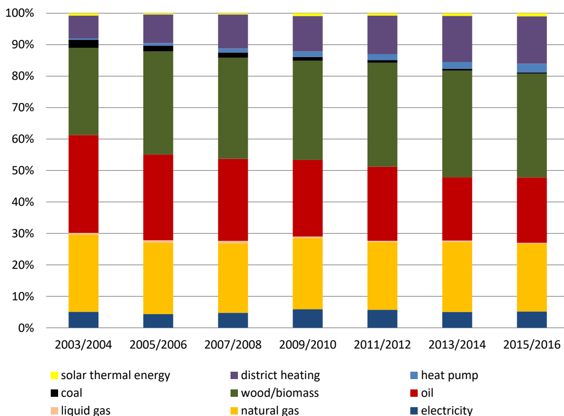
Figure 28: Relative use of energy sources for SH in all buildings; data according to Statistik Austria (2017)
