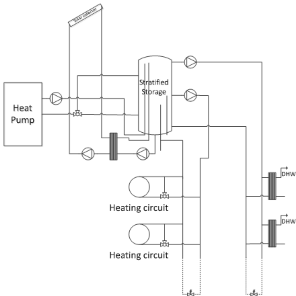
Figure 6: Simplified scheme of the hydraulic layout with a fresh water module in each dwelling (Green Heat Pump, 2014)
