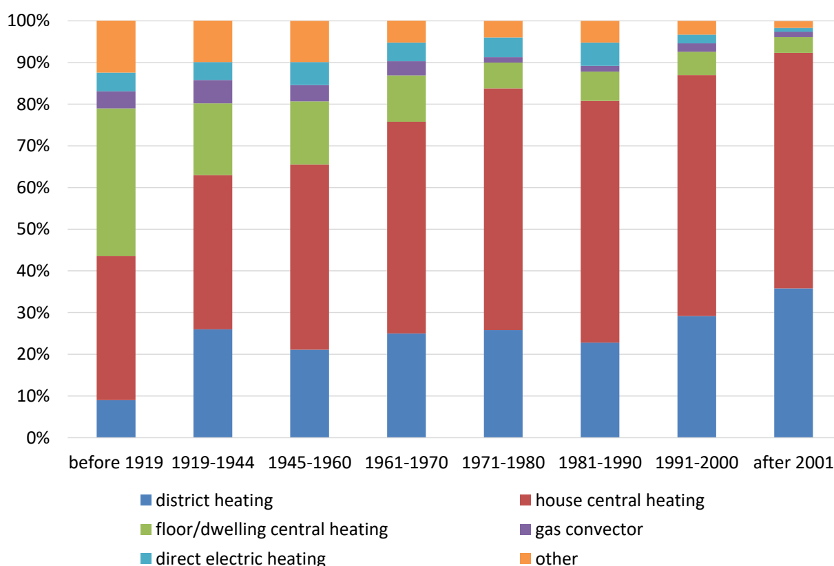
Figure 21: Heating systems in the building stock according to the construction period; data according to Statistik Austria (2016)
