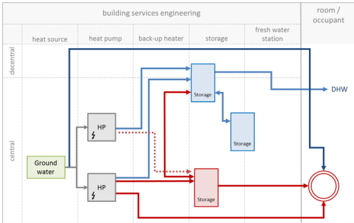
Figure 54: System layout of the system in Simmering
