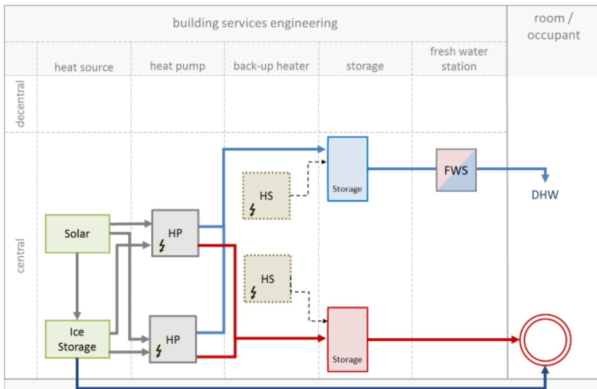
Figure 64: System layout of the system in Weiz
