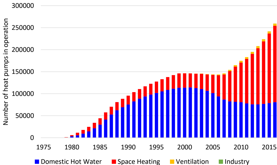
Figure 32: Number of heat pumps in operation in Austria; data according to Biermayer et al. (2017)
