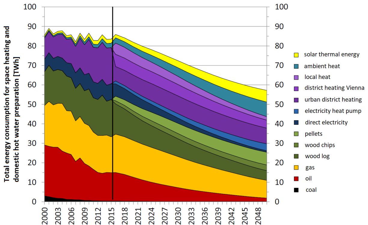
Figure 30: Forecast of the development of the energy demand till 2050 Müller et al. (2017) – translated
