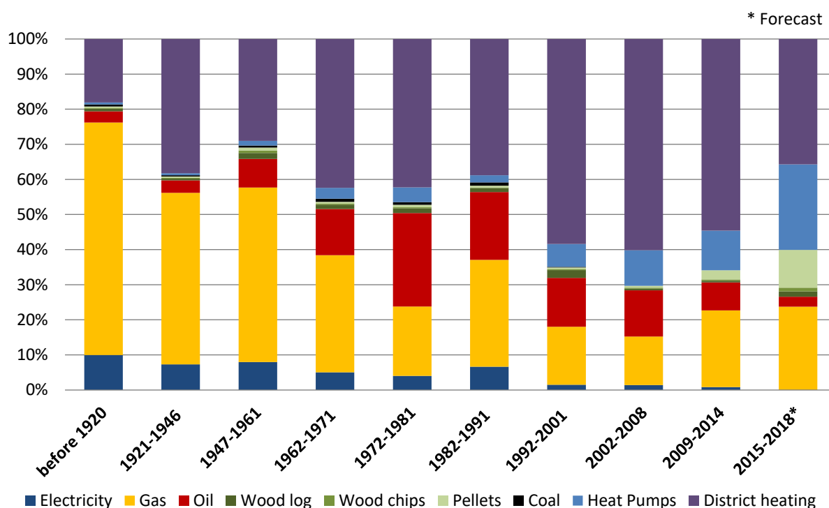
Figure 26: Share of used fuel types for heating in MFHs related to the heated gross floor area; data according to (Invert/EE-Lab Database, 2017)
