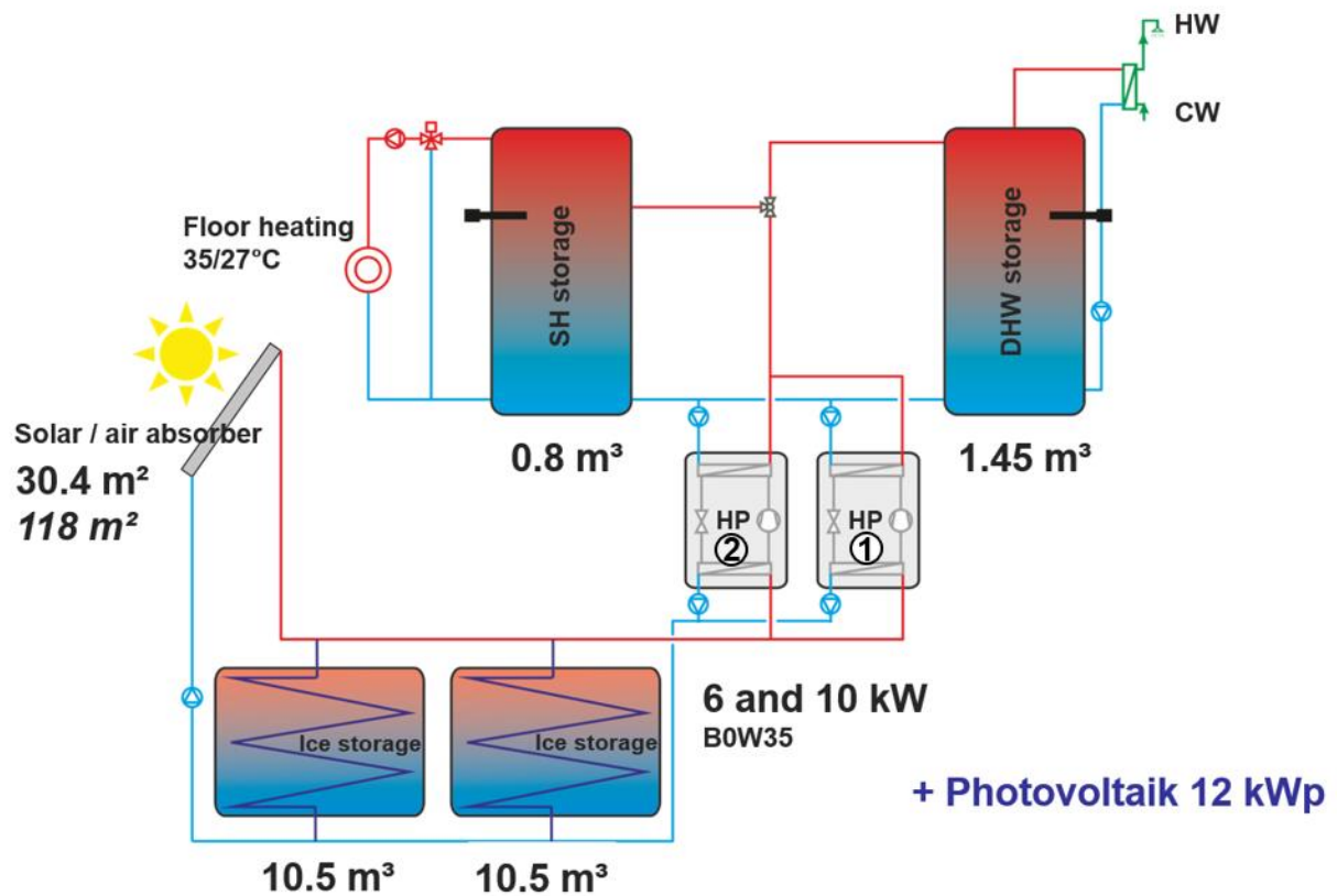
Figure 62: Hydraulic scheme (Pratter, 2017)
