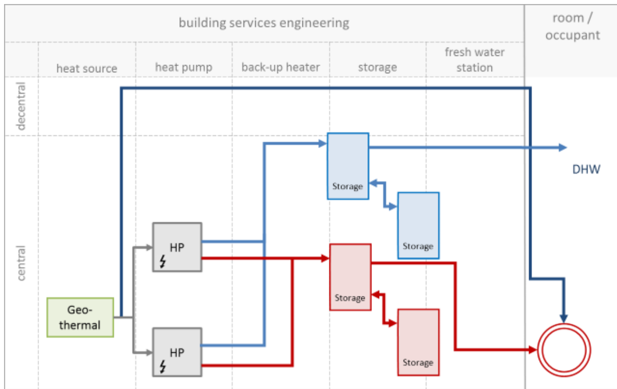
Figure 60: System layout of the system in Villach
