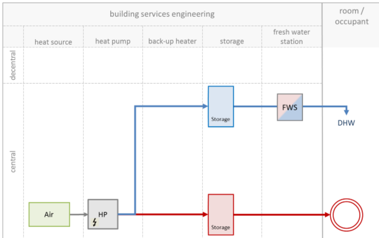
Figure 57: System layout of the system in Wien Praterstraße
