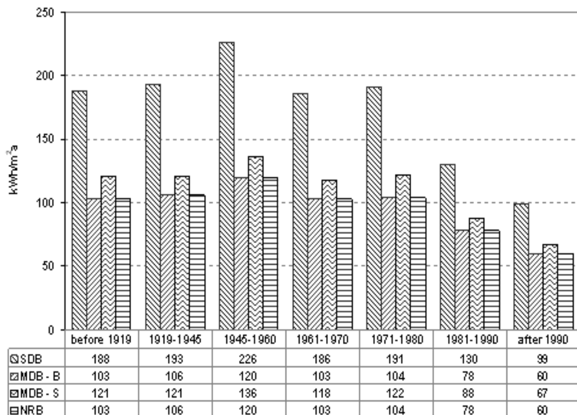
Figure 20: Specific annual energy use for heating in kWh/(m 2 *a) of single (SDB) and multi-dwellings (MDB; -B = Large, -S = Small) buildings, as well as non-residential buildings (NRB) by the construction period (Moisi et al., 2015)
