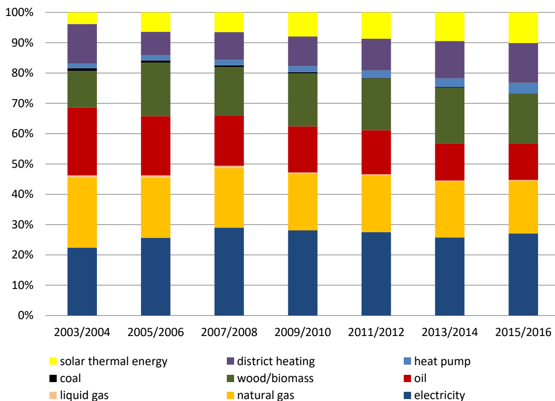
Figure 29: Relative usage of all energy sources for DHW heating; data according to Statistik Austria (2017)
