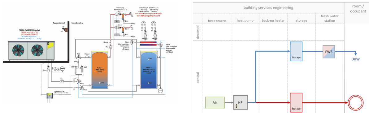
Figure 46: Example for a classic and IEA Annex 50 system layout
