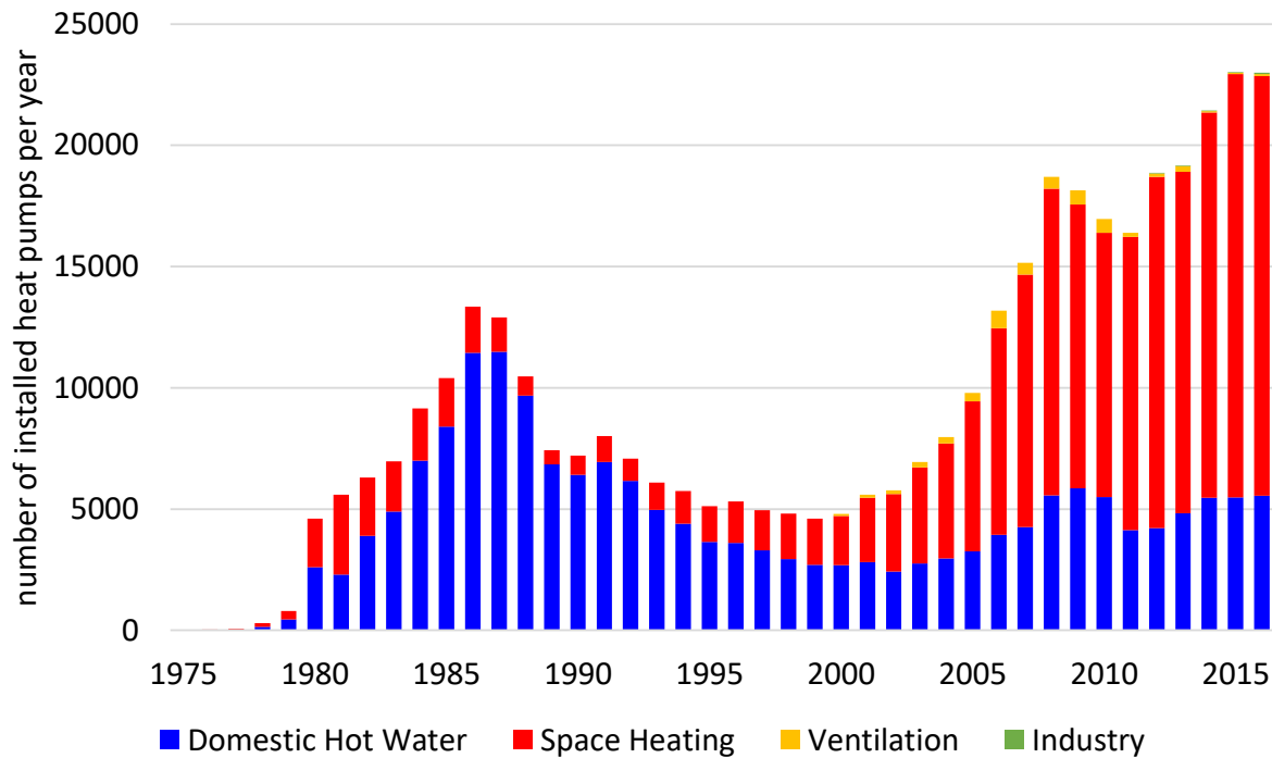
Figure 31: Number of installed heat pumps in Austria per year; data according to Biermayer et al. (2017)
