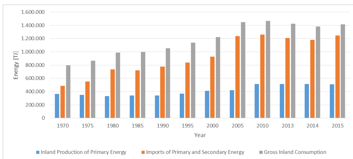
Figure 3: Austria's Inland Production of Primary Energy, Imports of Primary and Secondary Energy and Gross Inland Consumption between 1970 and 2015, diagram based on (Statistic Austria, 2015)
