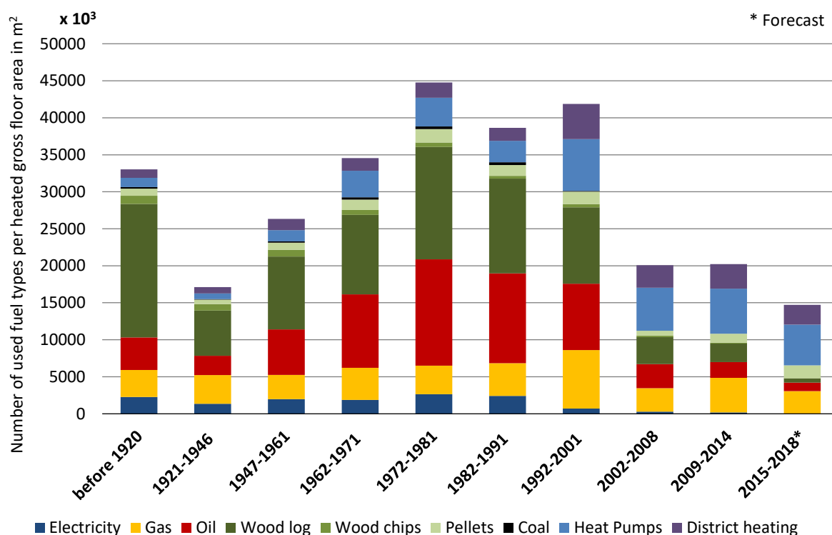
Figure 25: Number of used fuel types for heating per heated gross floor area in SFHs; data according to Invert/EE-Lab Database (2017)
