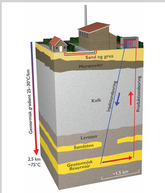
Fig 2: Overview of the geothermal district heating in Thisted. [GEUS].
